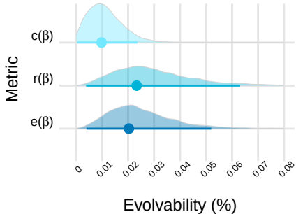
a) Trunk–Tail length
